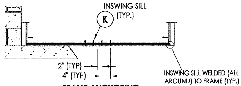
FRAME ANCHORING Direct to Masonry
