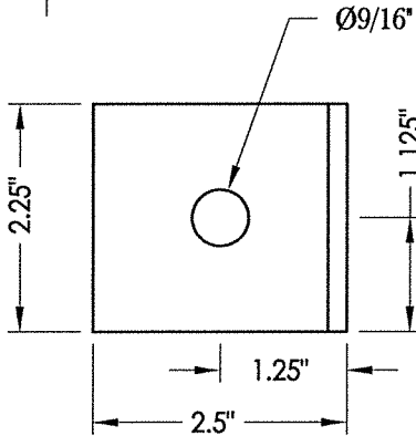
15 ANCHORING BRACKET
