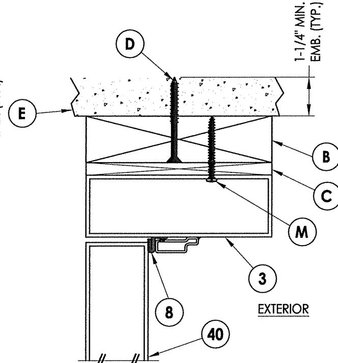
7 HORIZONTAL CROSS SECTION 3 Inswing Shown (Inswing Similar) 2X Buck Masonry Anchoring
