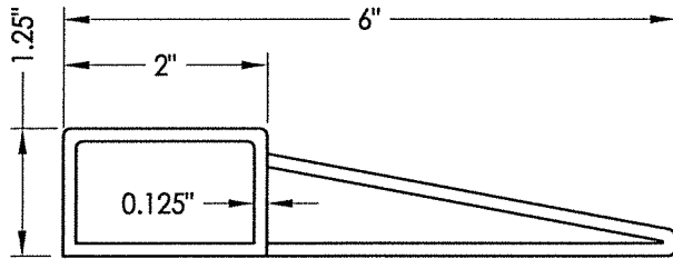
36 THRESHOLD Inswing
