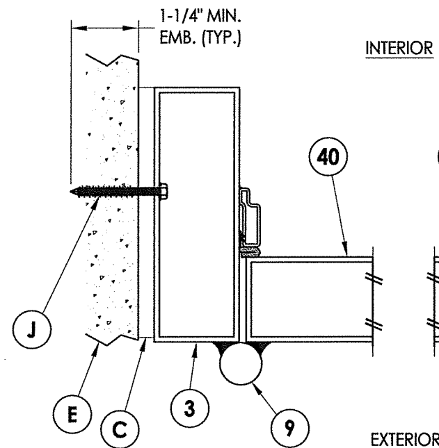
1 HORIZONTAL CROSS SECTION 3 Outswing Shown (Inswing Similar) Direct to Masonry Anchoring
